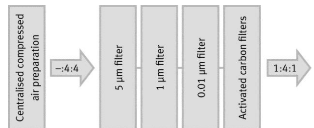
Filter cascade for compliance with class 1:4:1
