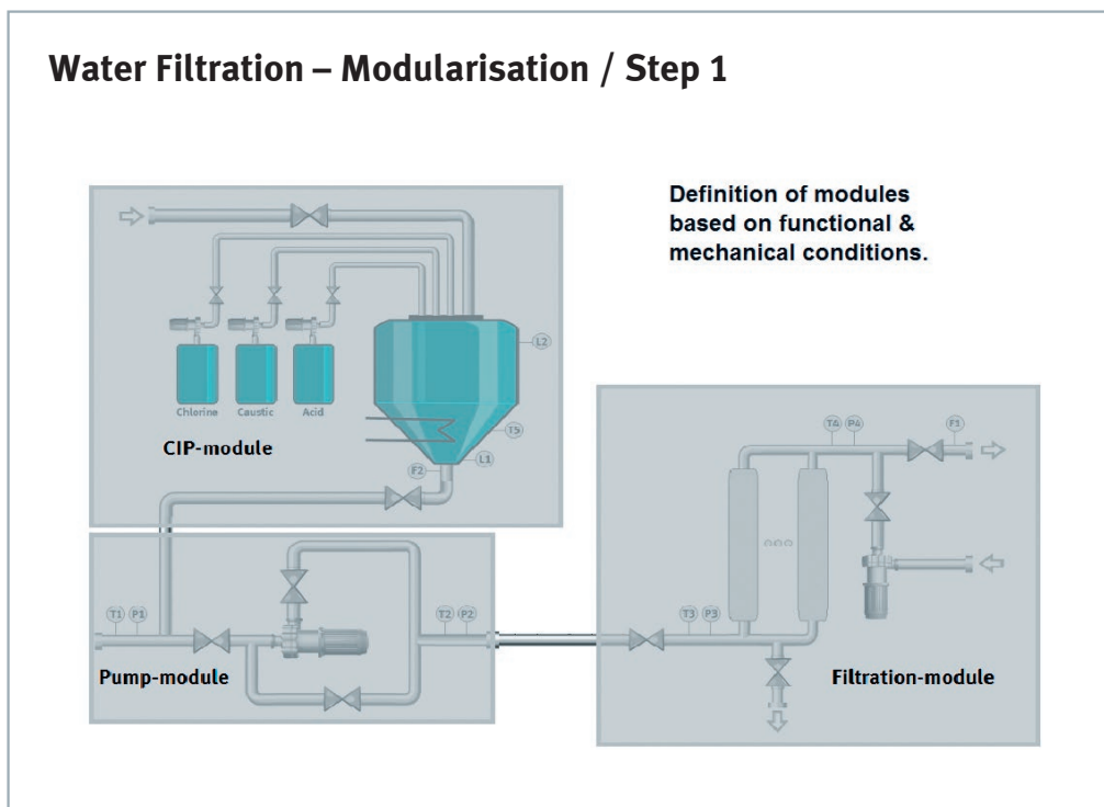
Figure 2: Modularisation of the mechanical and functional tasks of a water filtration plant
