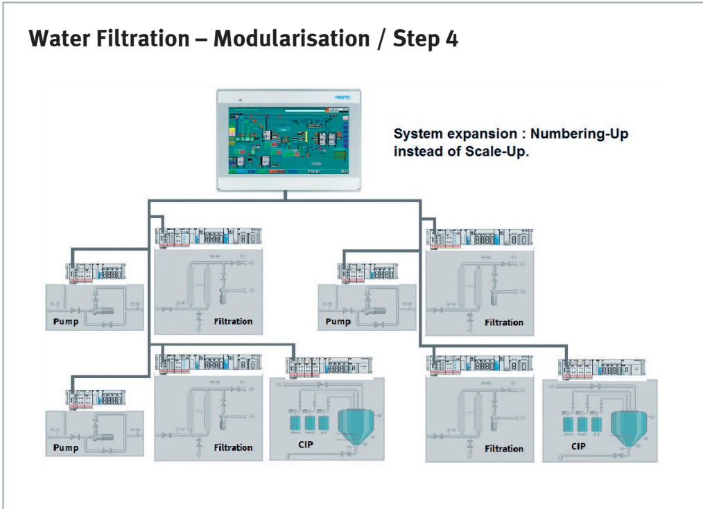
Figure 5: System expansion by numbering up
