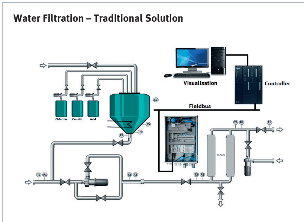
Figure 1: Traditional process plant design (water filtration plant)
