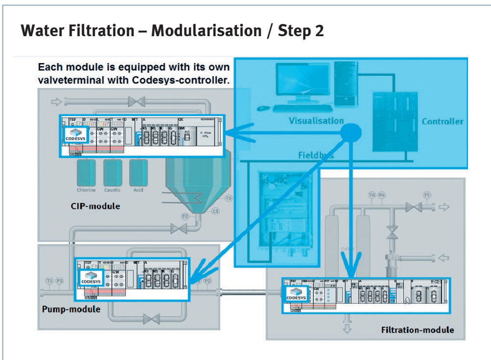
Figure 3: Modularisation of the automation tasks of a water filtration plant
